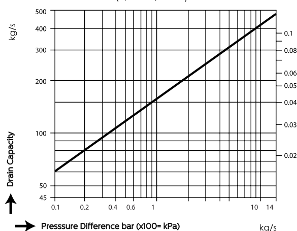
Drain Capacities (1/2" - 3/4" - 1")
